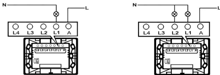
1 Gang Switch
