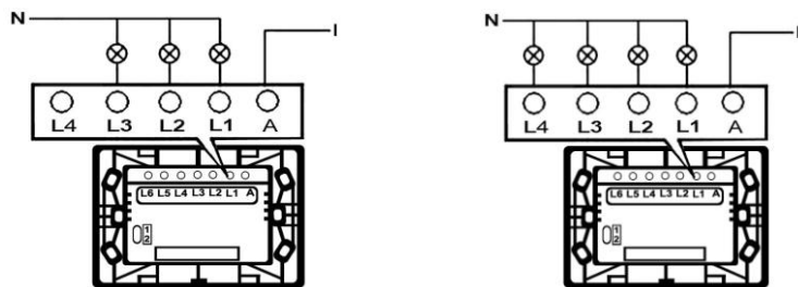
3 Gang Switch
